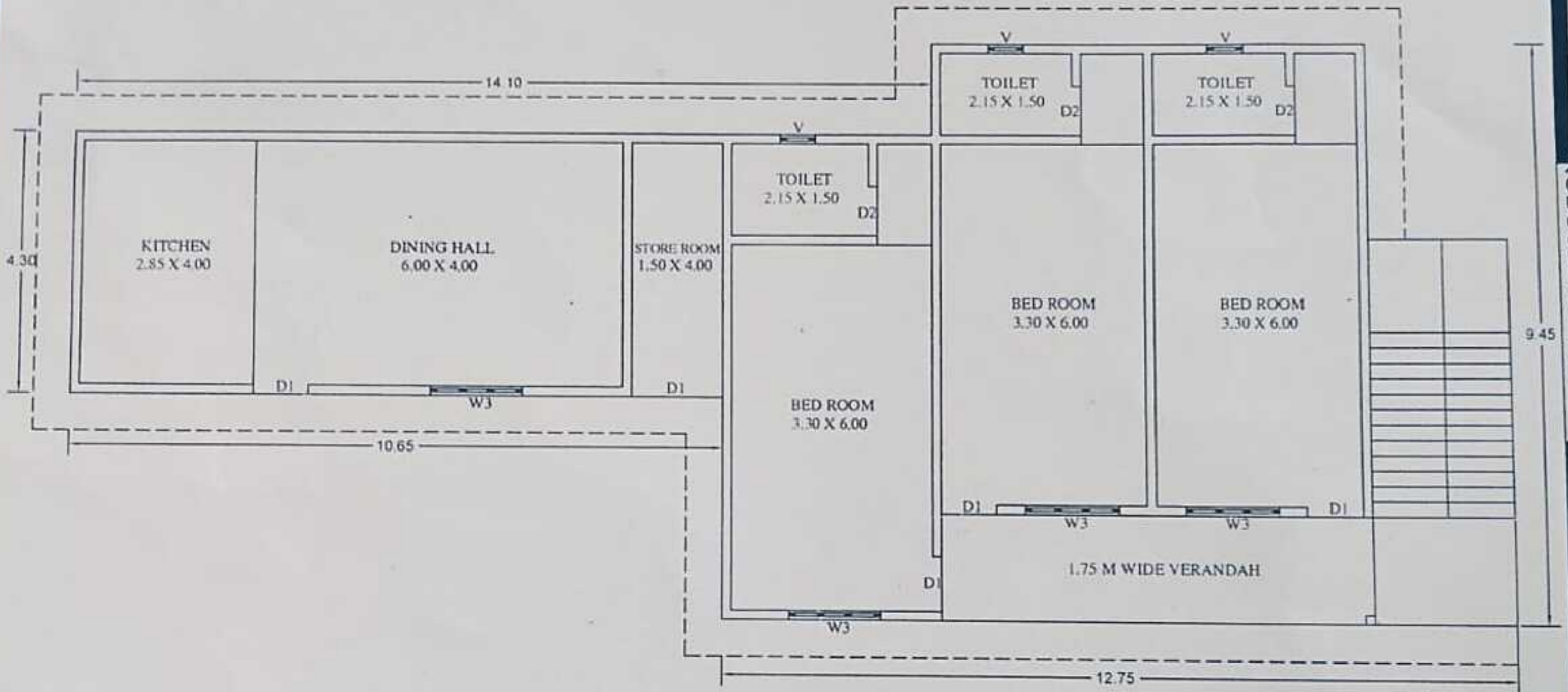
BUILDING PLAN
