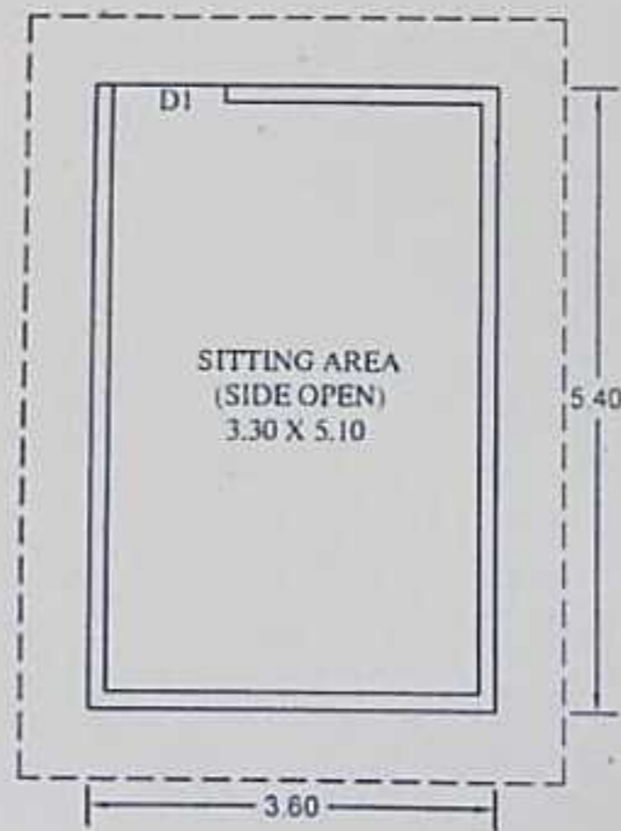
BUILDING PLAN
